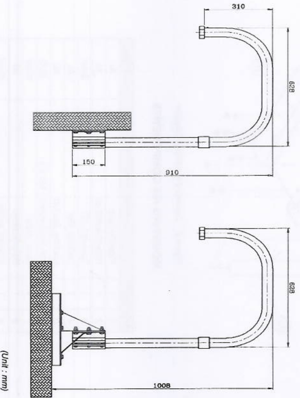
Figure 3. Dimension Drawing
