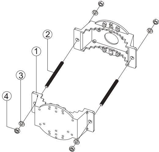
[ POLE MOUNT ASS'Y - EXPLODED VIEW ]
