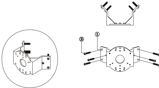
[ INSTALLING PLATE AT THE WALL ]
