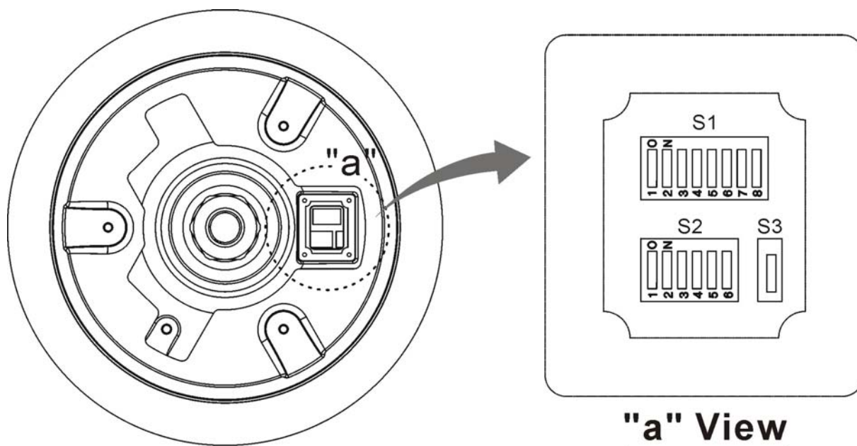
Figure 2 – Layout of DIP Switches
