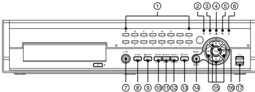
Figure 3 — 16-Channel DVR front panel.
