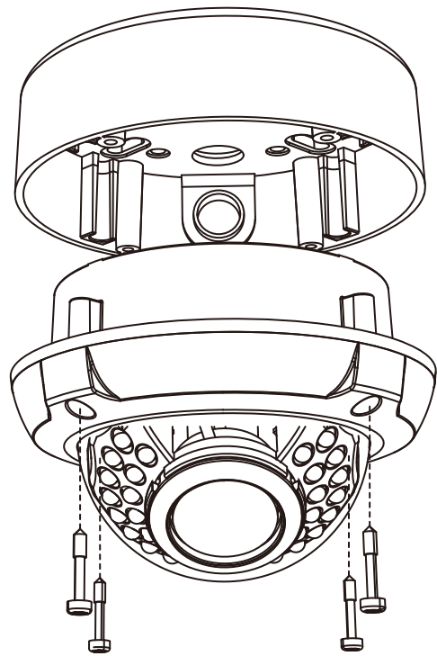
M4 Machine screw x 4 (supplied)
