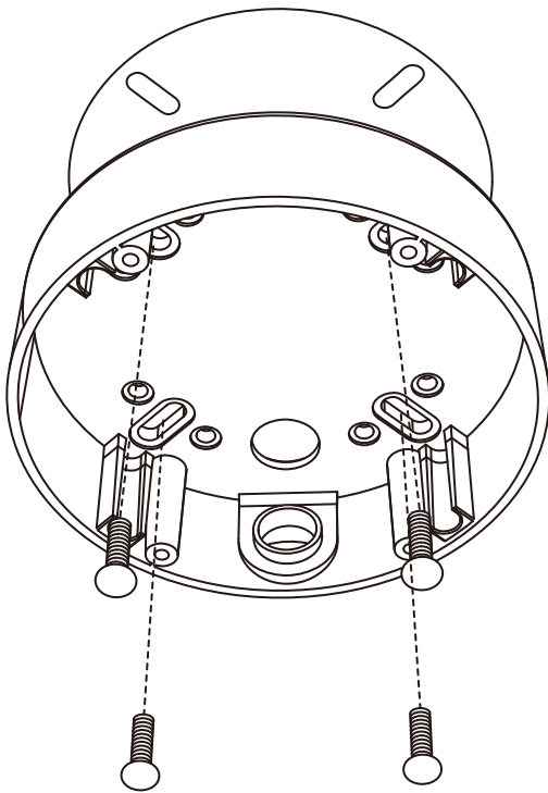
Ø5 tapping screw x 4 (supplied)
