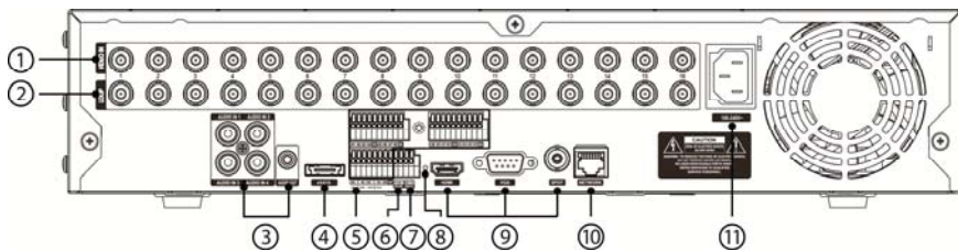
Figure 2: DVR rear panel.
